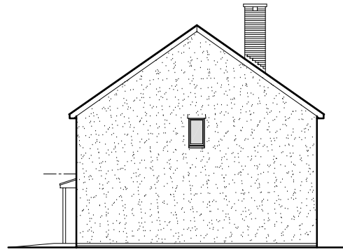
SIDE ELEVATION (1:200)
