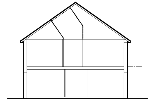
TYPICAL SECTION (1:200)
